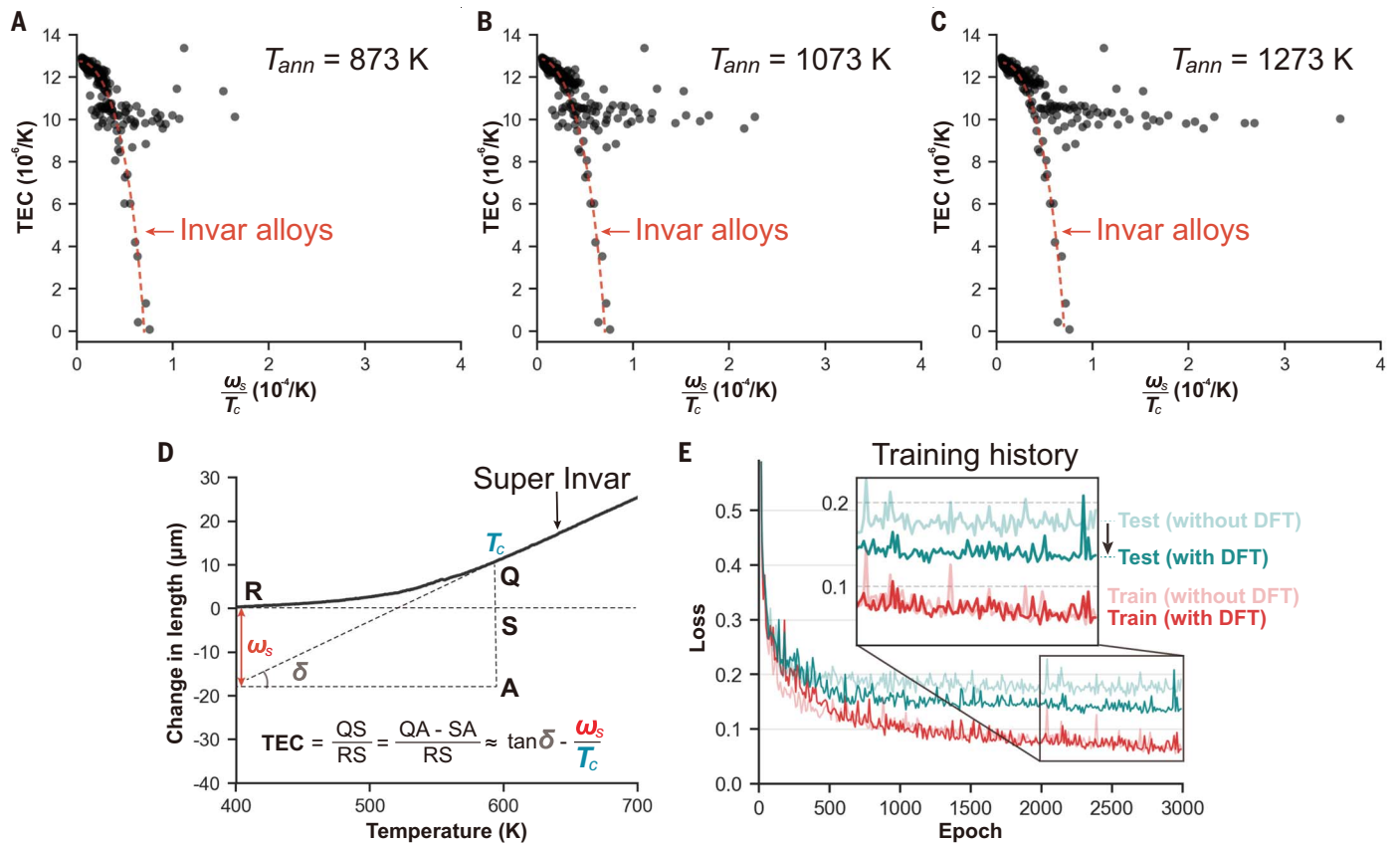
Fig. 3. Importance of the physics-informed descriptors. (A–C) Correlation between the proposed descriptor \omega_s/T_c and the experimental TEC. (D) Schematic model of the Masumoto empirical rule for discovering Invar alloys. (E) Comparison of training and testing history with and without use of the descriptor \omega_s/T_c . Both the final training and testing errors decrease after considering the physics-informed descriptors; for example, the testing error decreases from 19 to 14%.
